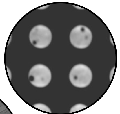
Interior BGA Voiding
